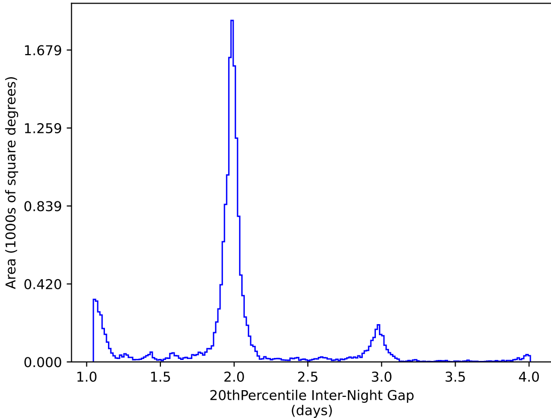
weather_cloudso1v3.4_10yrs WFD y band: 20thPercentile Inter-Night Gap
