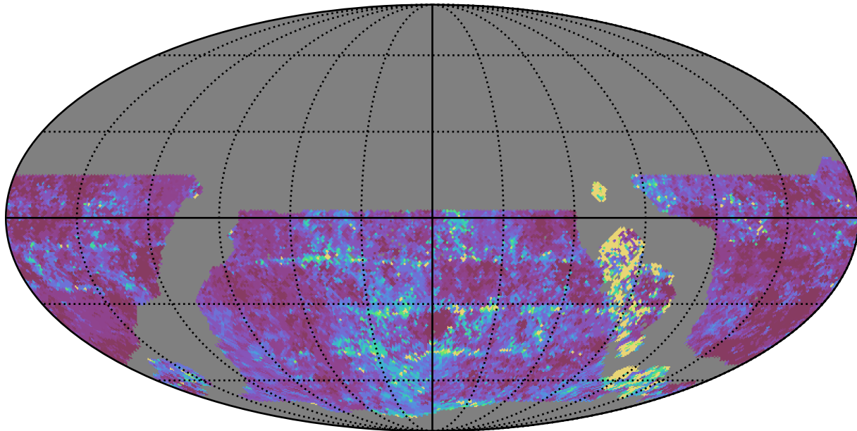
weather_cloudso1v3.4_10yrs WFD u band: 20thPercentile Inter-Night Gap
