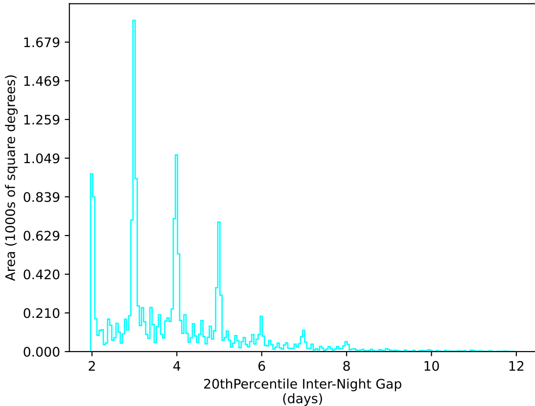
weather_cloudso1v3.4_10yrs WFD u band: 20thPercentile Inter-Night Gap
