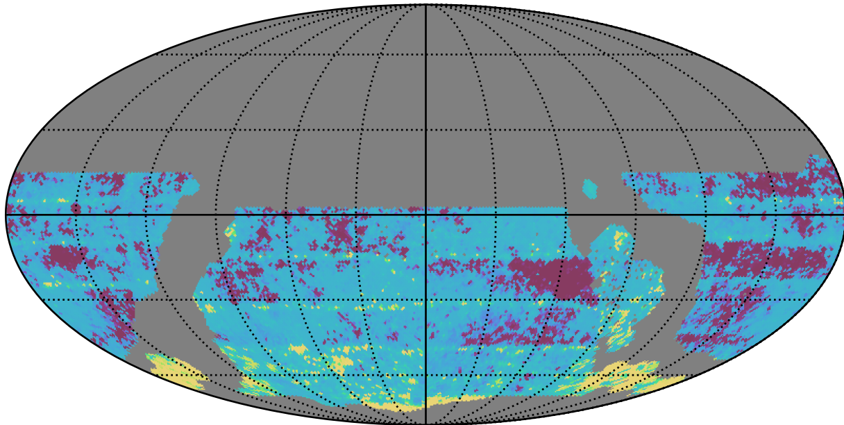
weather_cloudso1v3.4_10yrs WFD r band: 20thPercentile Inter-Night Gap
