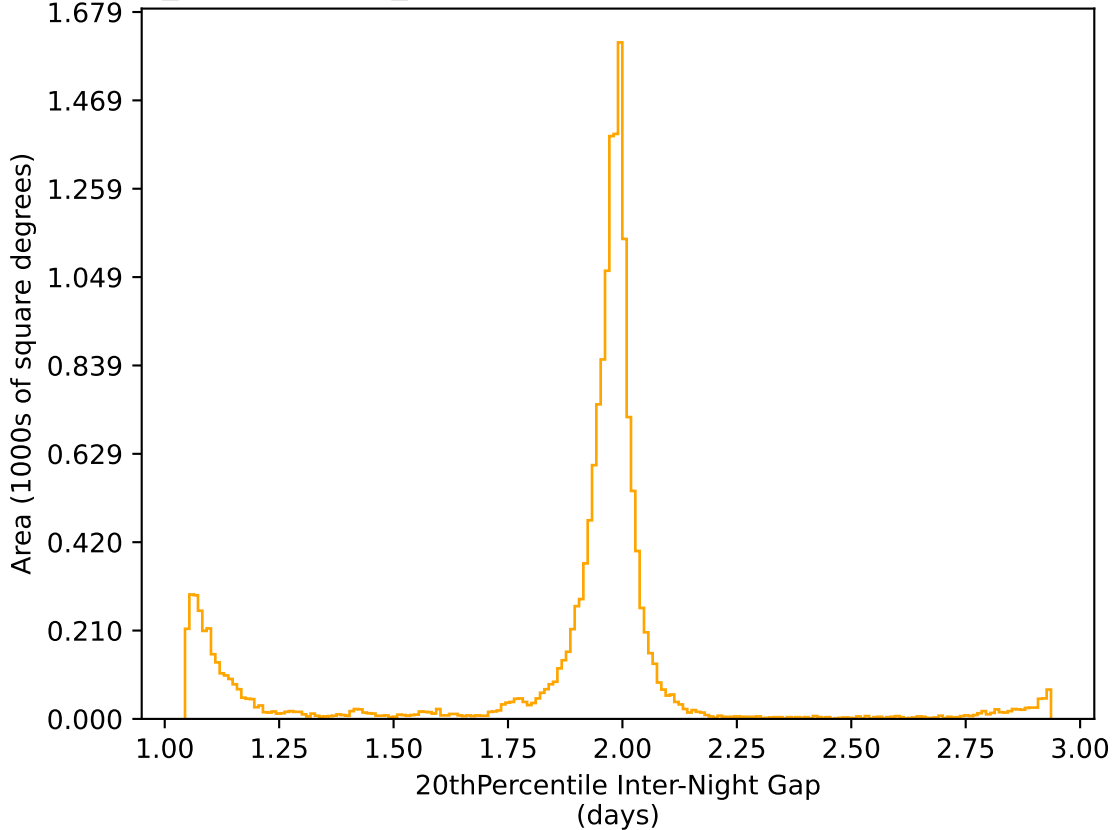
weather_cloudso1v3.4_10yrs WFD r band: 20thPercentile Inter-Night Gap
