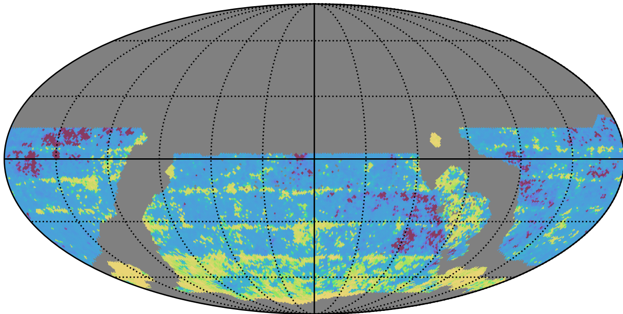
weather_cloudso1v3.4_10yrs WFD i band: 20thPercentile Inter-Night Gap
