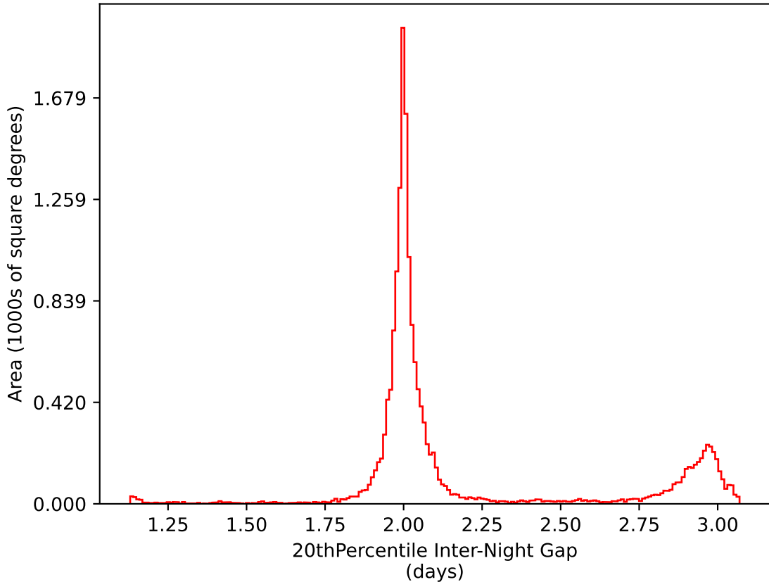
weather_cloudso1v3.4_10yrs WFD i band: 20thPercentile Inter-Night Gap
