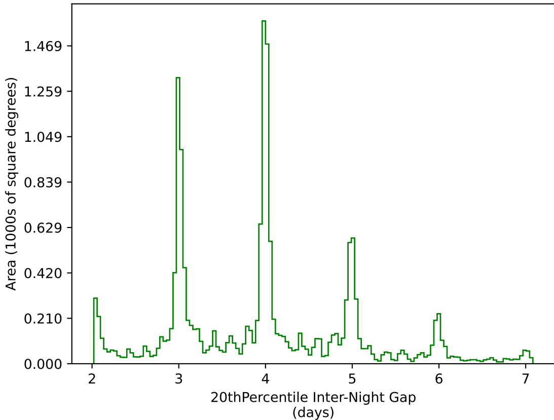
weather_cloudso1v3.4_10yrs WFD g band: 20thPercentile Inter-Night Gap
