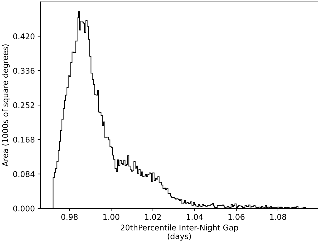
weather_cloudso1v3.4_10yrs WFD all bands: 20thPercentile Inter-Night Gap
