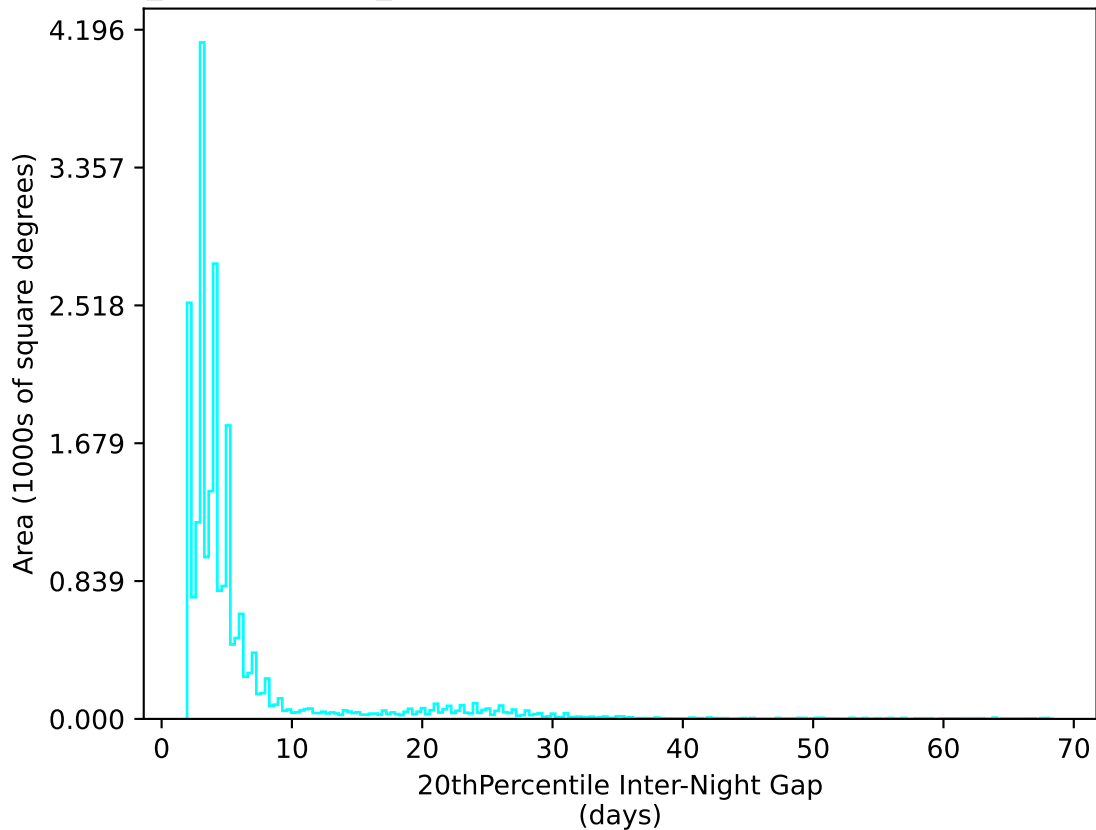
weather_cloudso1v3.4_10yrs All sky u band: 20thPercentile Inter-Night Gap
