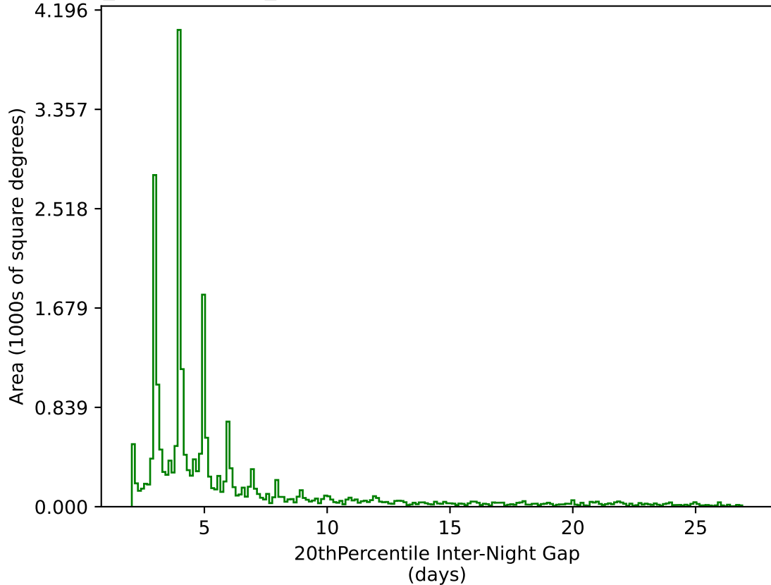
weather_cloudso1v3.4_10yrs All sky g band: 20thPercentile Inter-Night Gap
