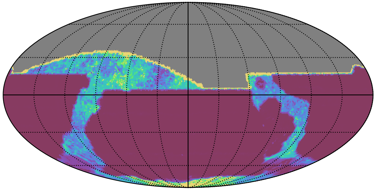
weather_cloudso1v3.4_10yrs All sky all bands: 20thPercentile Inter-Night Gap
