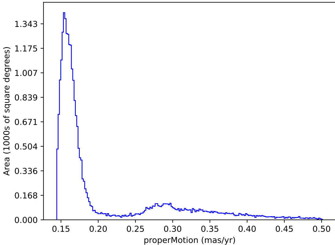
weather_cloudso1v3.4_10yrs : properMotion
