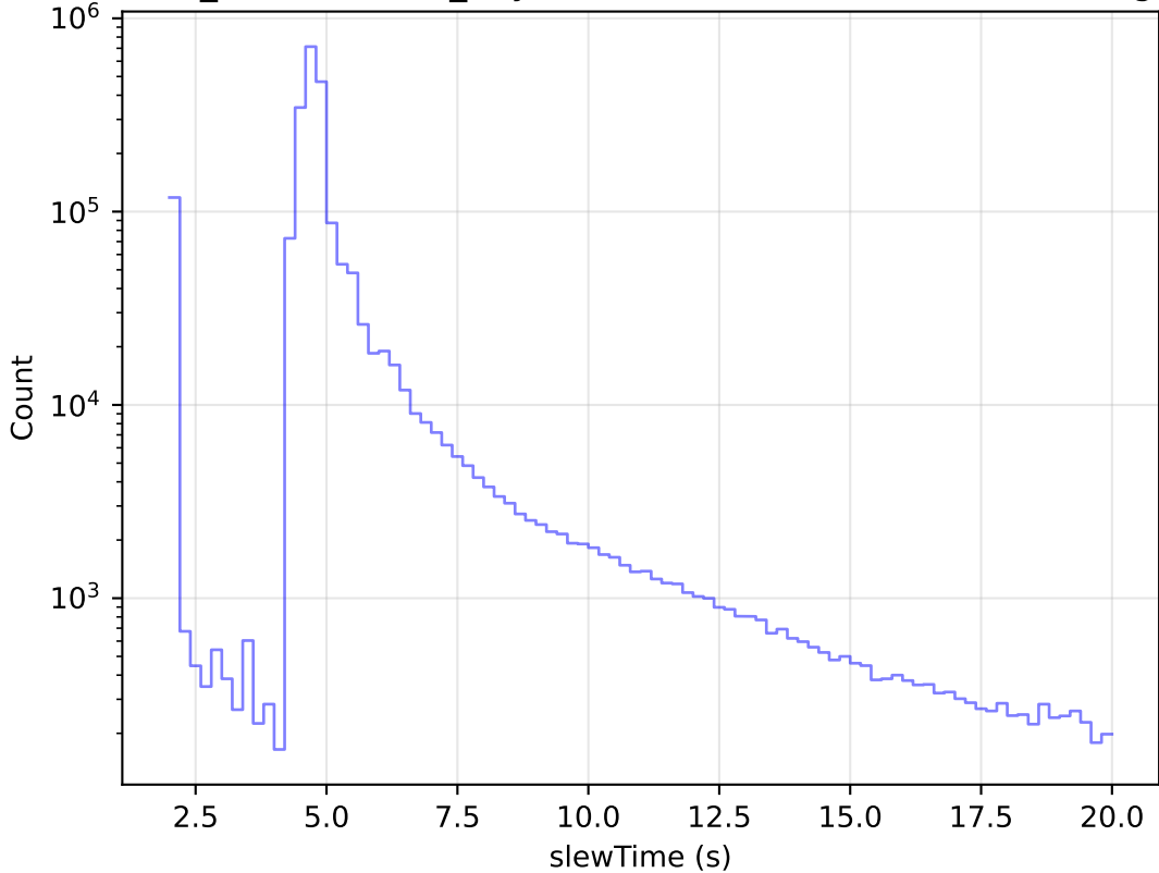
weather_cloudso1v3.4_10yrs All visits: Zoom Slew Time Histogram
