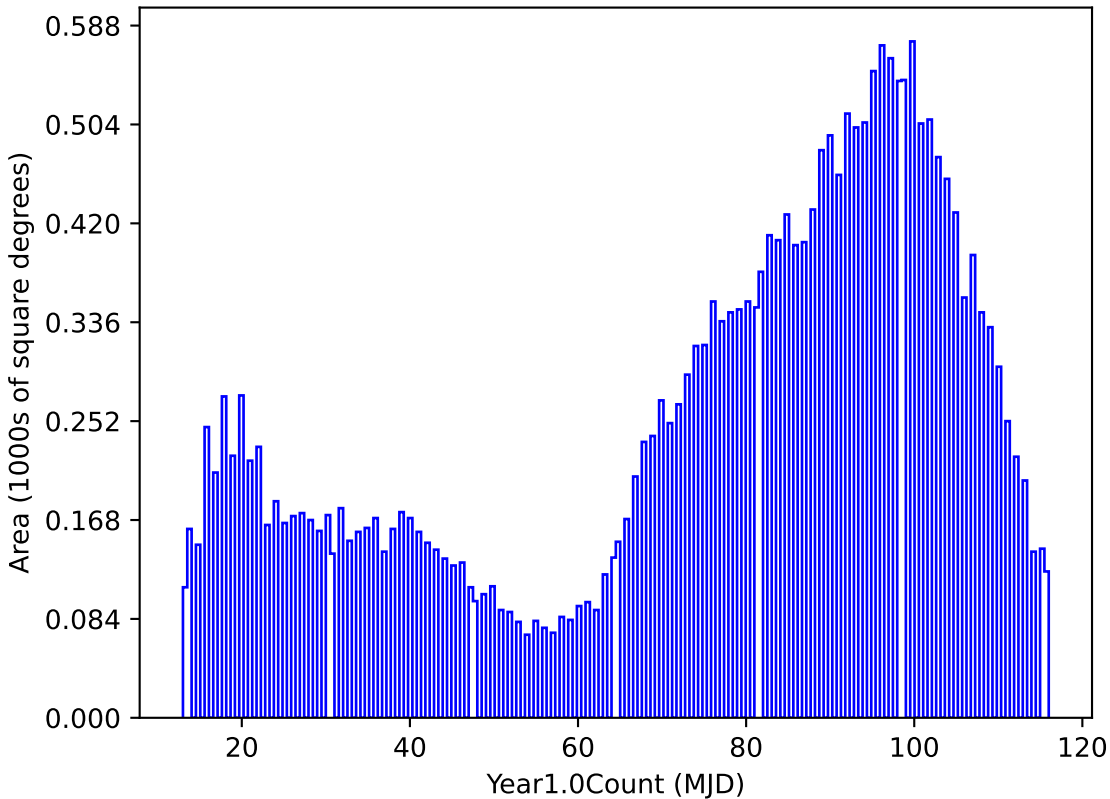
weather_cloudso1v3.4_10yrs night < 365.25: Year1.0Count
