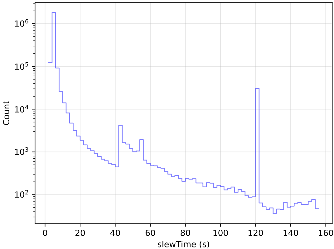
weather_cloudso1v3.4_10yrs All visits: Slew Time Histogram
