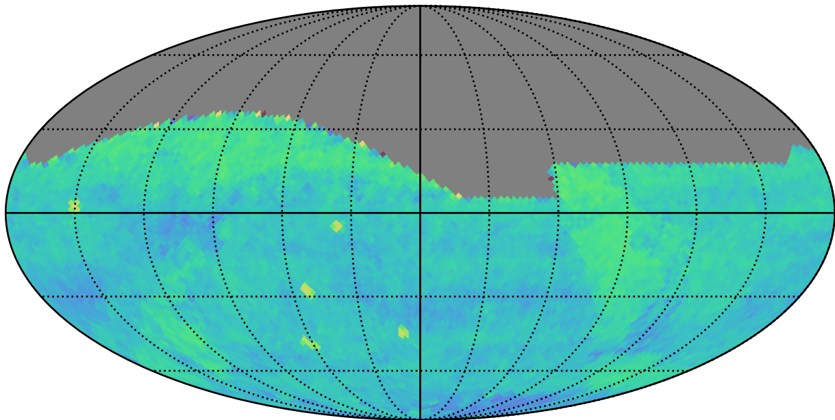
weather_cloudso1v3.4_10yrs (g or r or i): PairFraction
