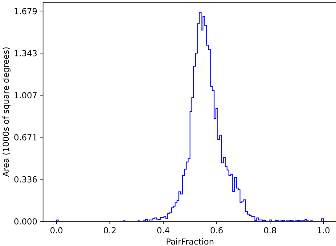
weather_cloudso1v3.4_10yrs (g or r or i): PairFraction
