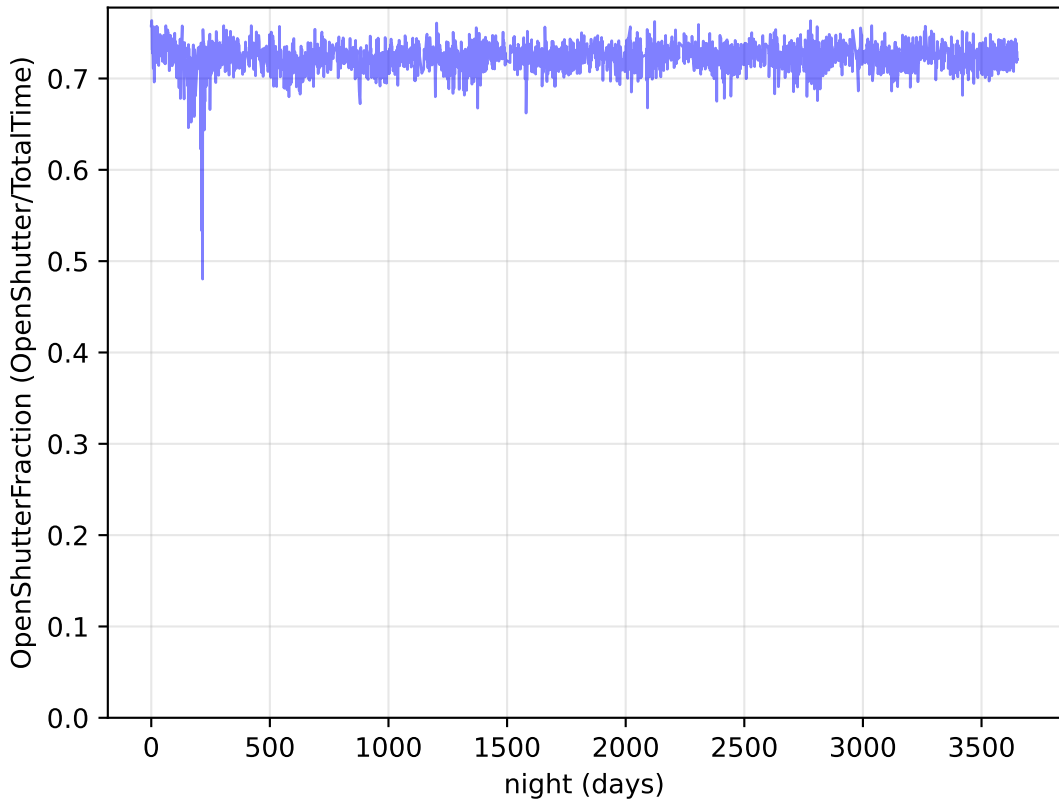
weather_cloudso1v3.4_10yrs : OpenShutterFraction
