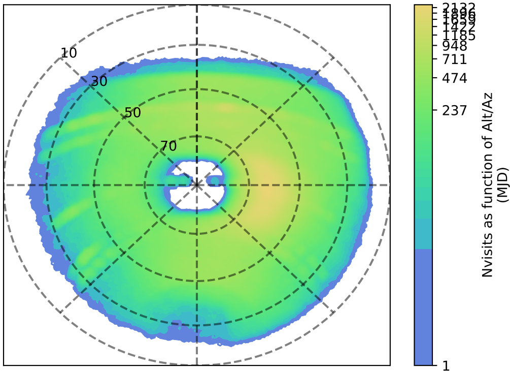
weather_cloudso1v3.4_10yrs y: Nvisits as function of Alt/Az
