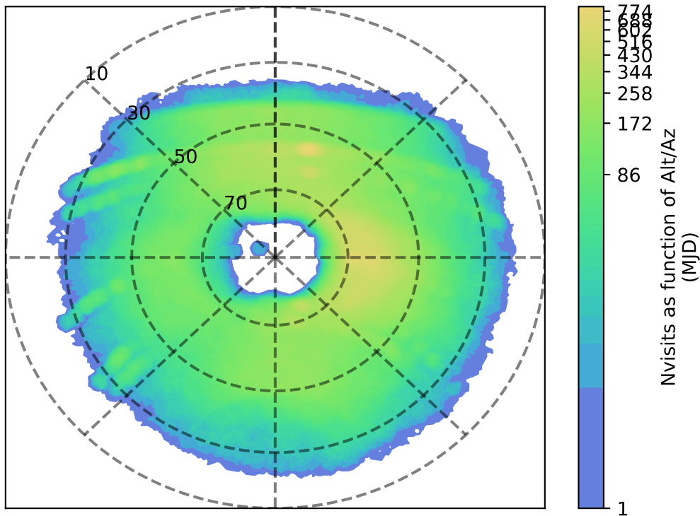
weather_cloudso1v3.4_10yrs u: Nvisits as function of Alt/Az
