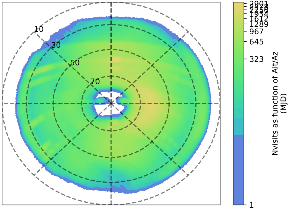
weather_cloudso1v3.4_10yrs i: Nvisits as function of Alt/Az
