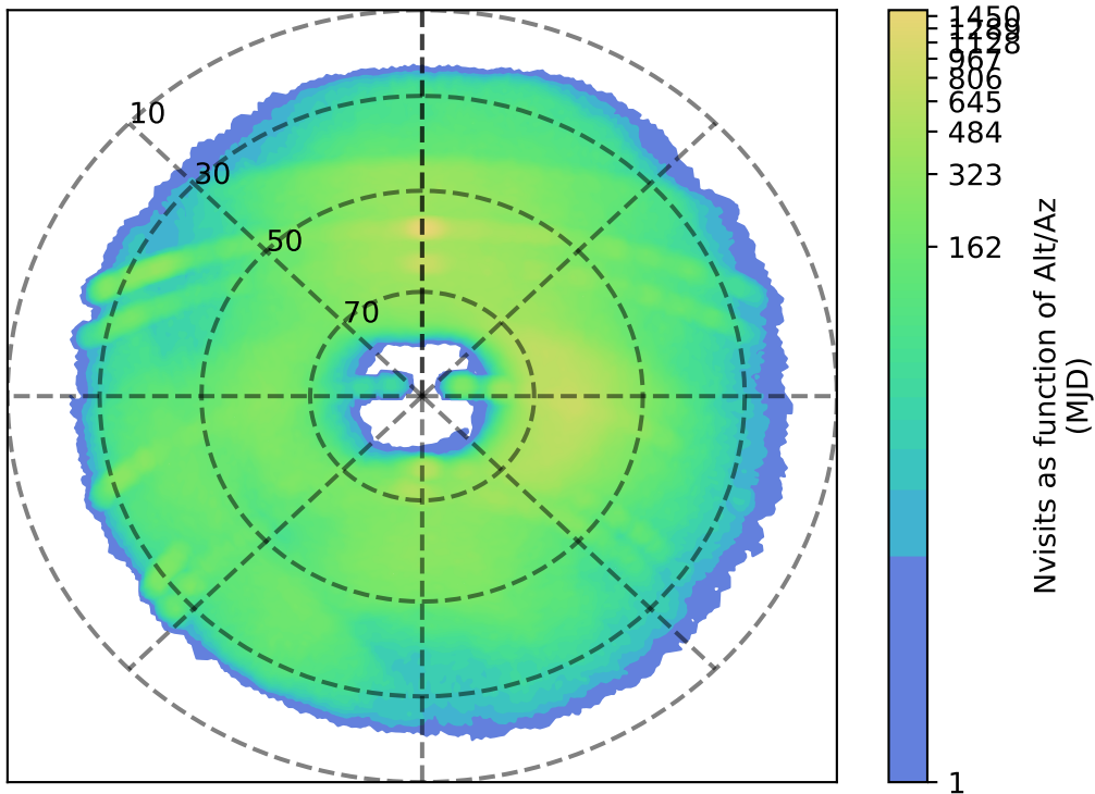
weather_cloudso1v3.4_10yrs g: Nvisits as function of Alt/Az
