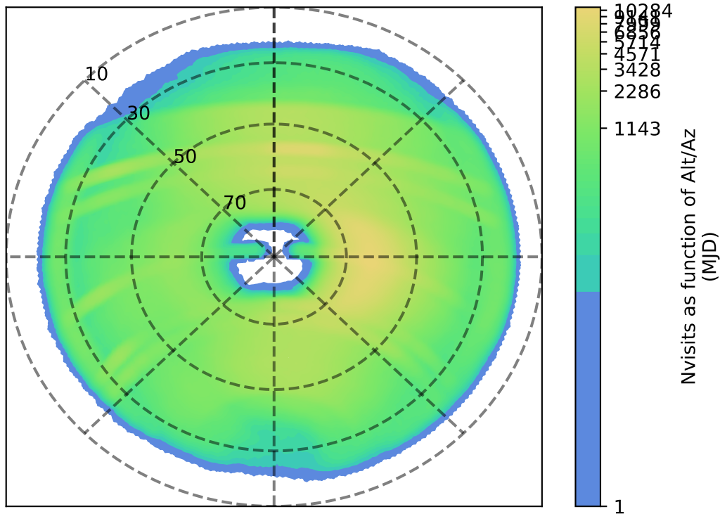
weather_cloudso1v3.4_10yrs : Nvisits as function of Alt/Az
