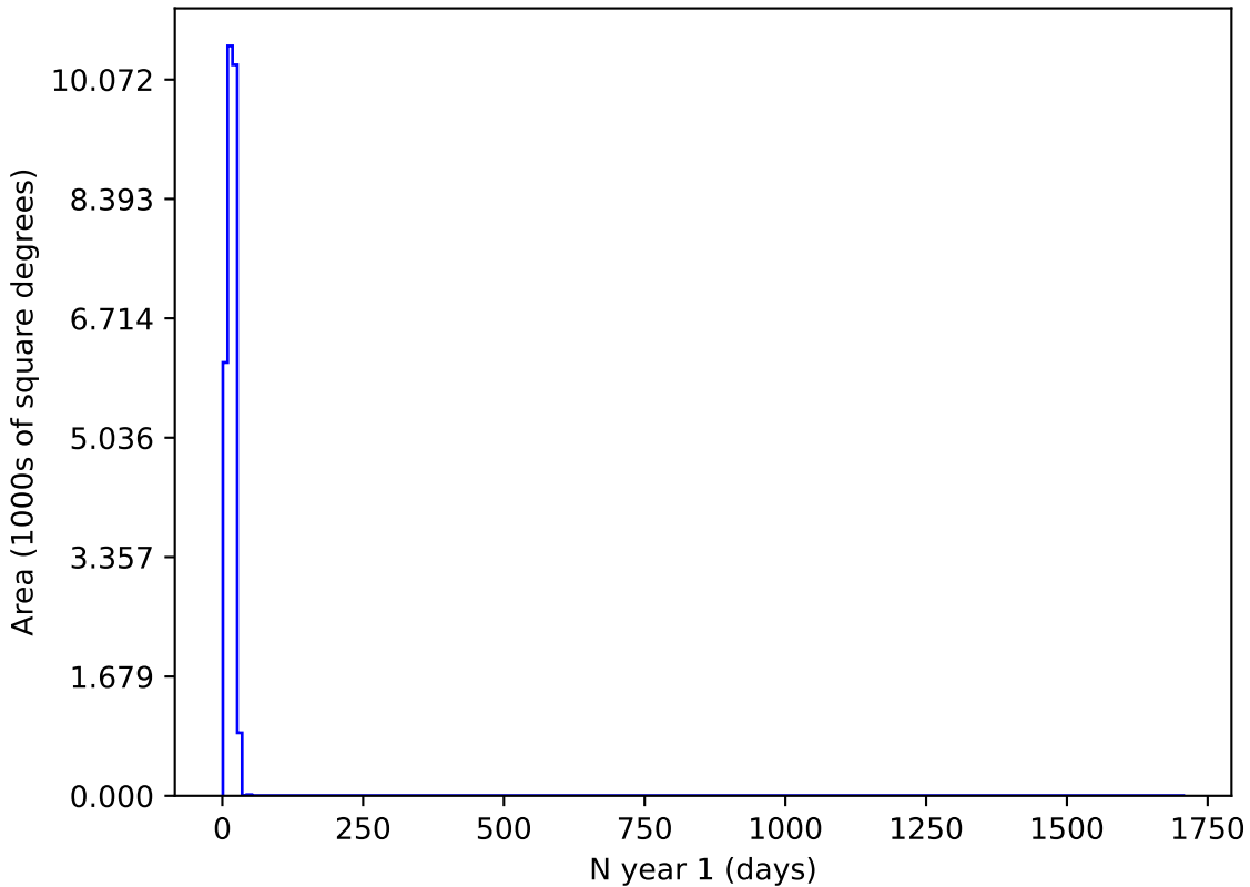
weather_cloudso1v3.4_10yrs r and night < 365: N year 1
