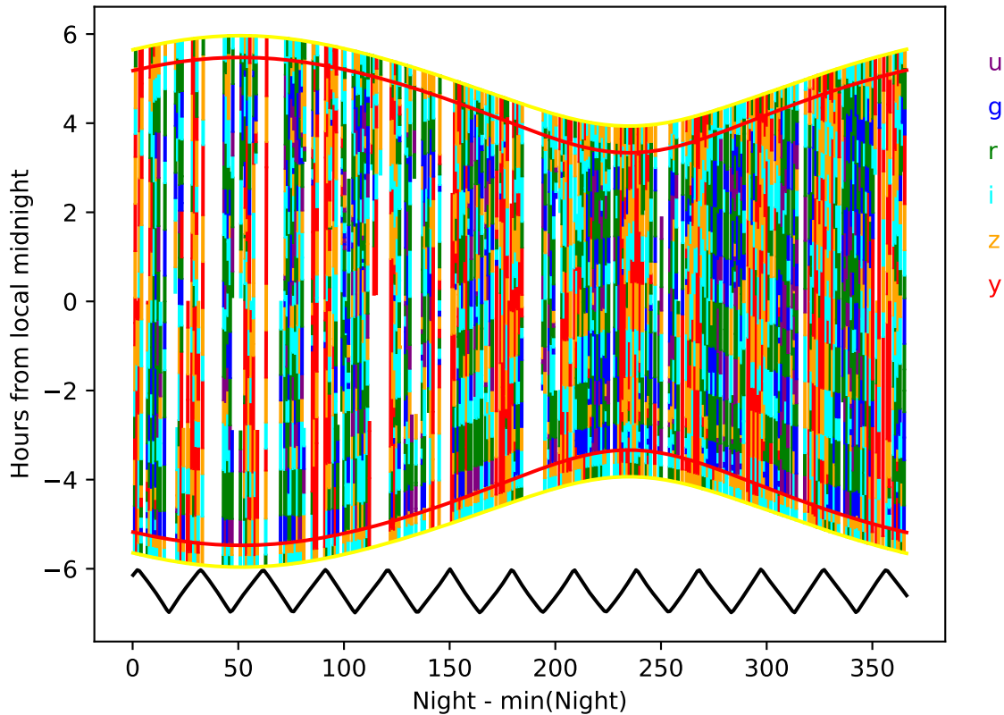
weather_cloudso1v3.4_10yrs year 9-10: Hourglass
