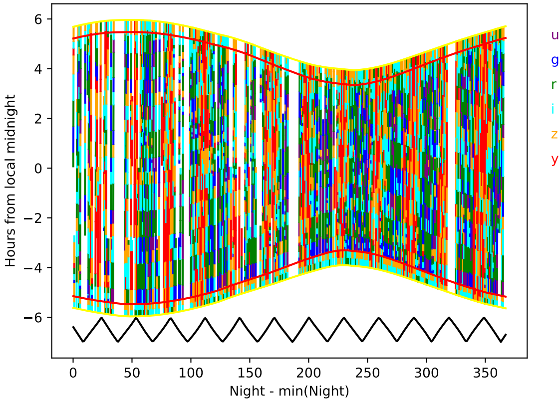
weather_cloudso1v3.4_10yrs year 7-8: Hourglass
