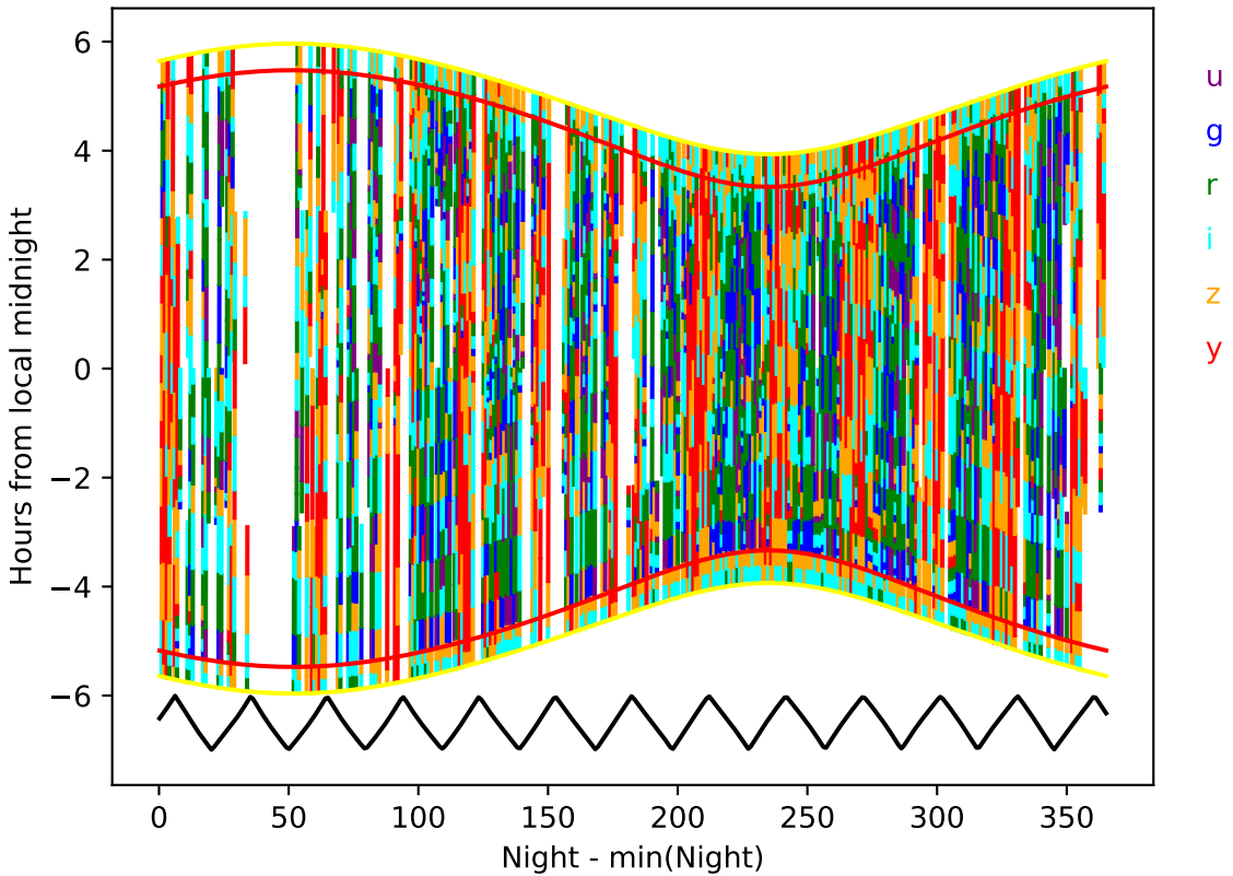
weather_cloudso1v3.4_10yrs year 6-7: Hourglass
