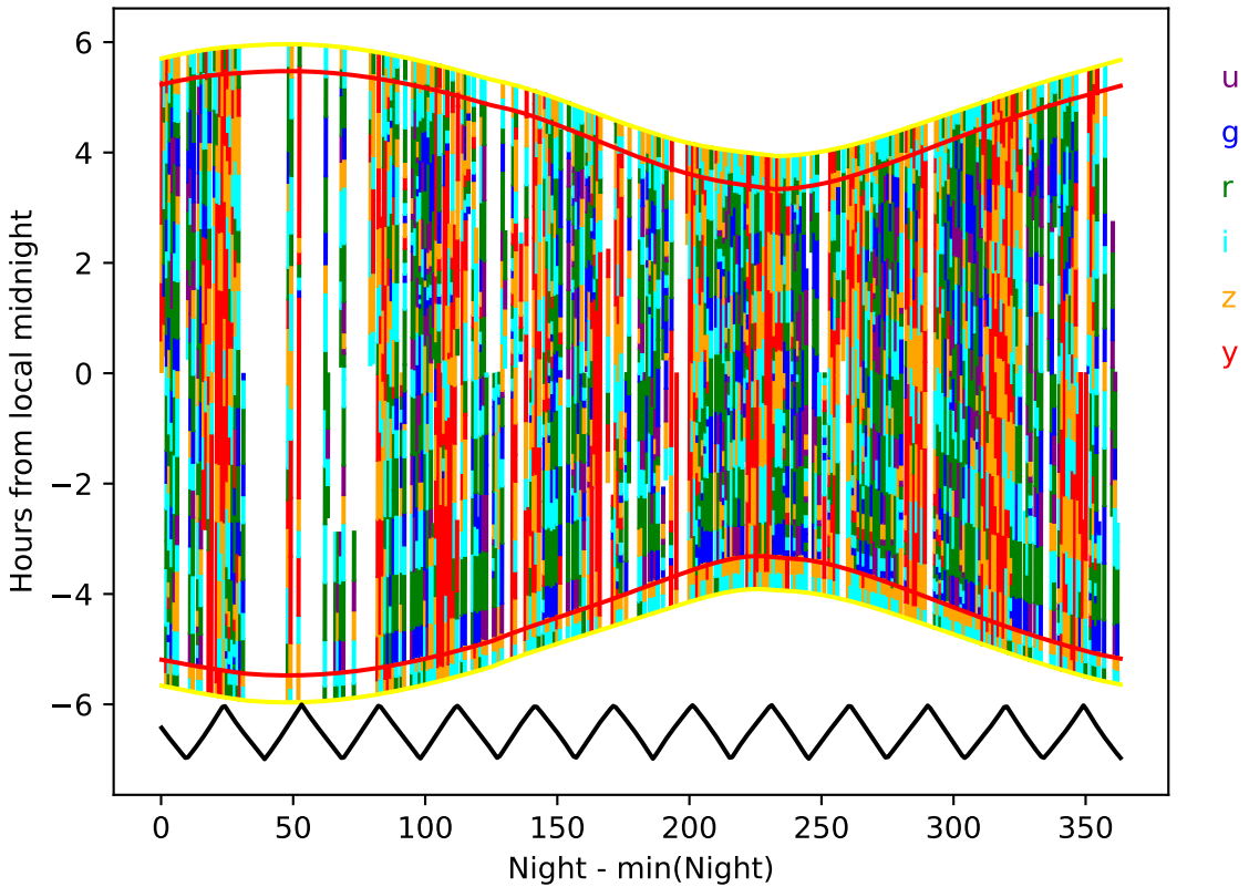
weather_cloudso1v3.4_10yrs year 4-5: Hourglass
