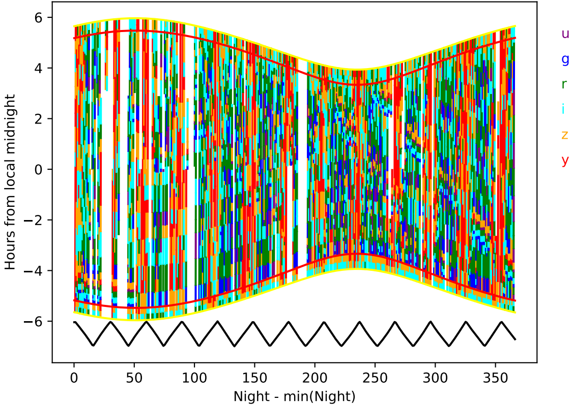
weather_cloudso1v3.4_10yrs year 1-2: Hourglass
