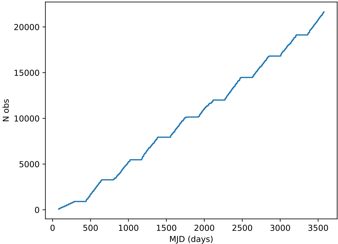
weather_cloudso1v3.4_10yrs note like DD:XMM_LSS%: Cumulative
