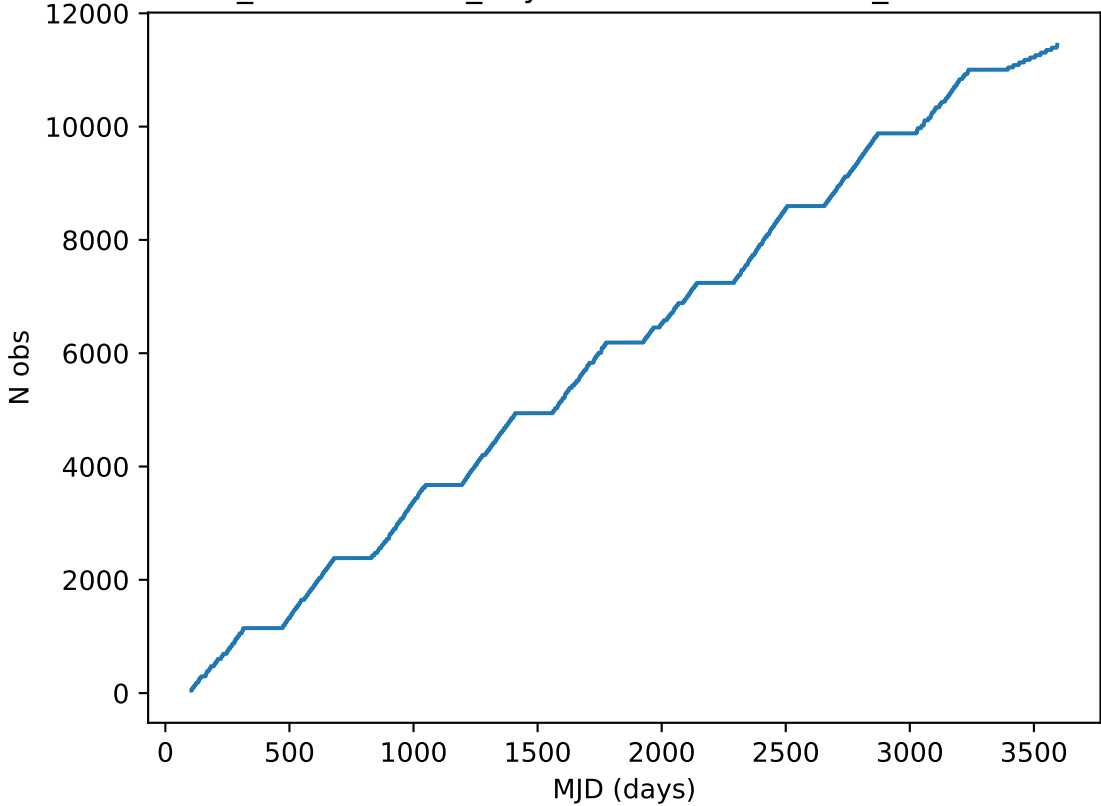
weather_cloudso1v3.4_10yrs note like DD:EDFS_b%: Cumulative
