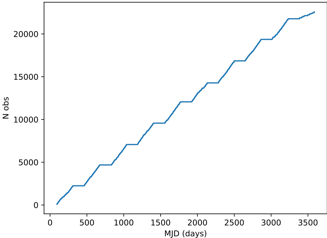
weather_cloudso1v3.4_10yrs note like DD:ECDFS%: Cumulative
