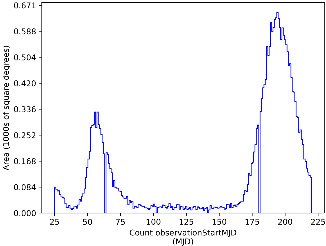
weather_cloudso1v3.4_10yrs i: Count observationStartMJD
