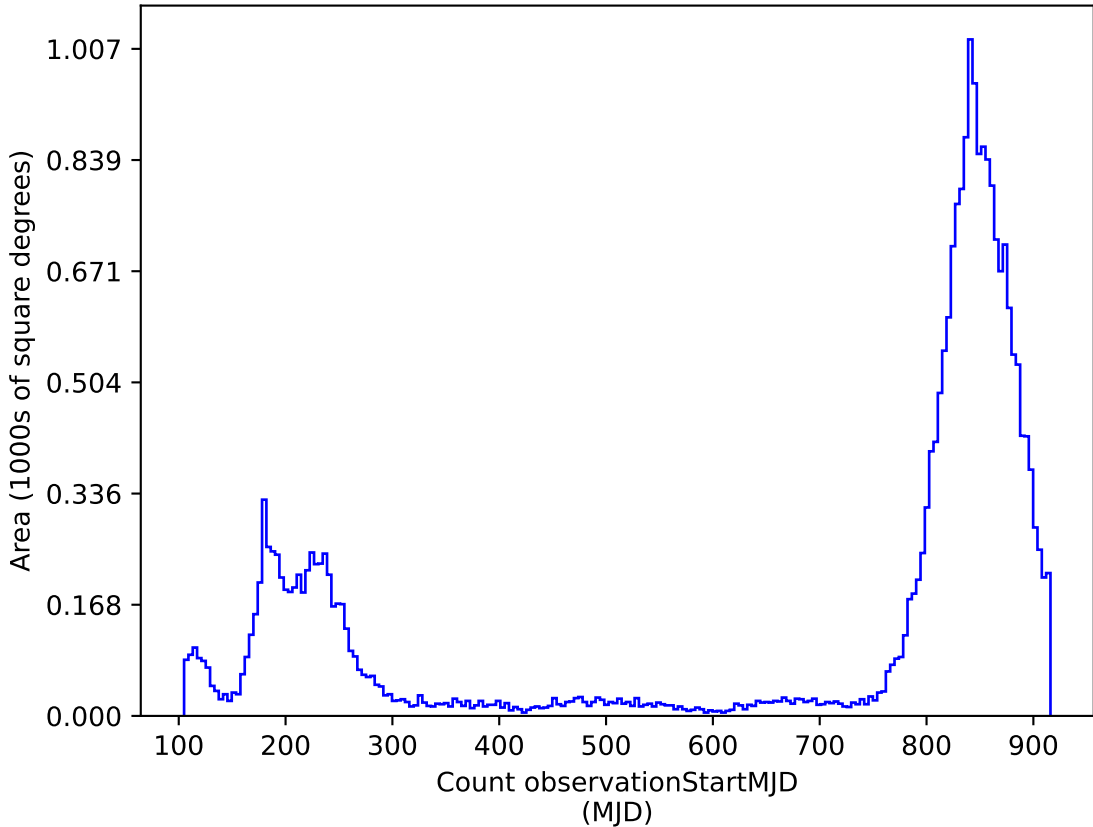
weather_cloudso1v3.4_10yrs : Count observationStartMJD
