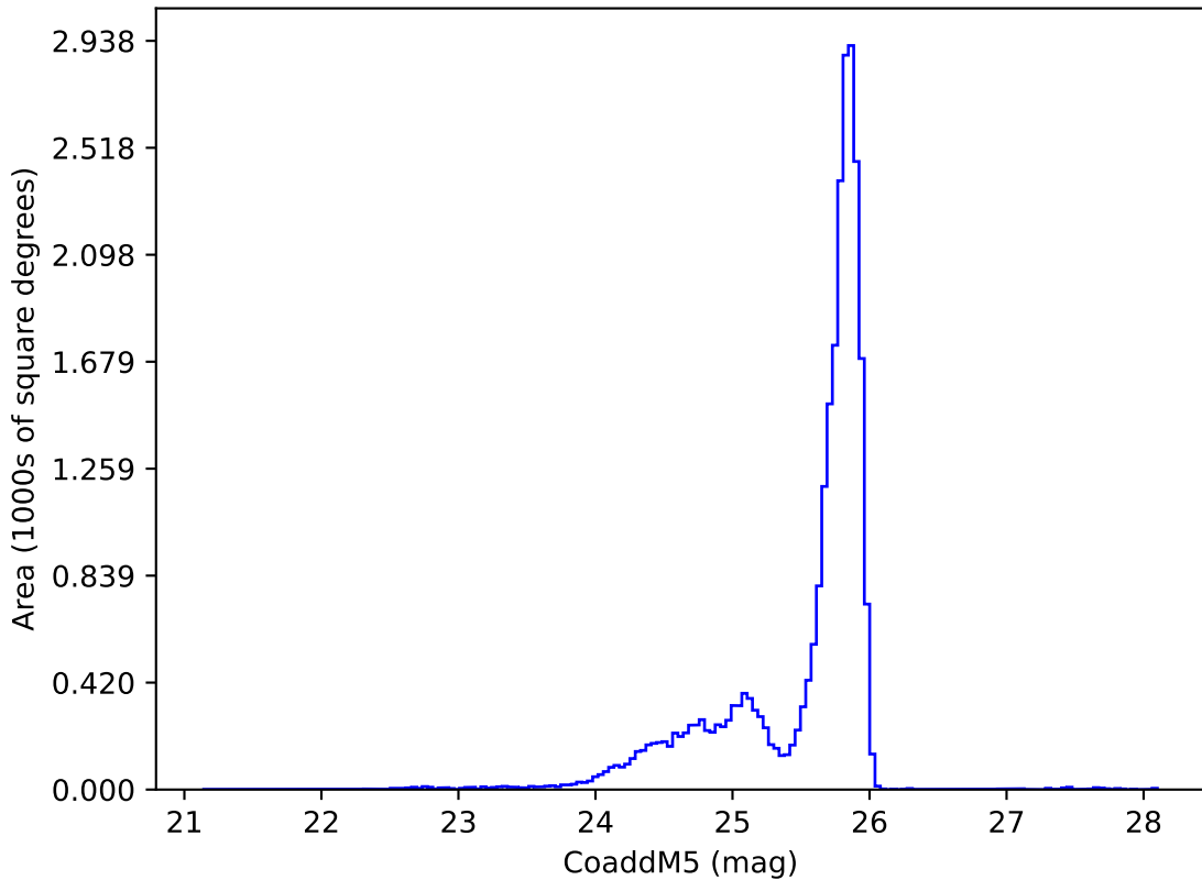
weather_cloudso1v3.4_10yrs z: CoaddM5
