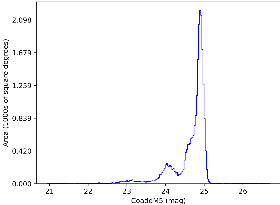
weather_cloudso1v3.4_10yrs y: CoaddM5
