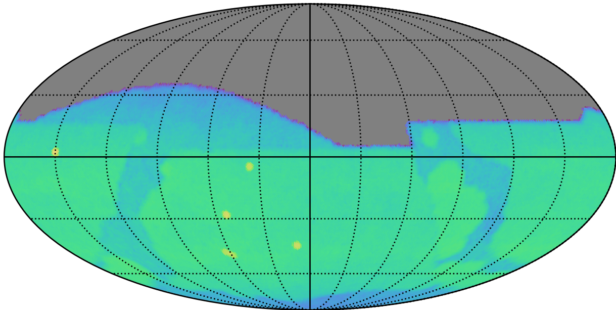
weather_cloudso1v3.4_10yrs g: CoaddM5
