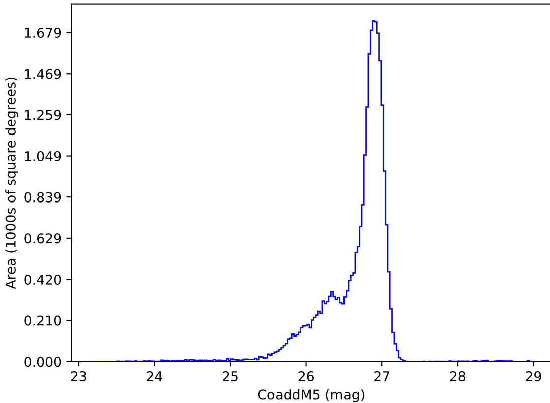
weather_cloudso1v3.4_10yrs g: CoaddM5
