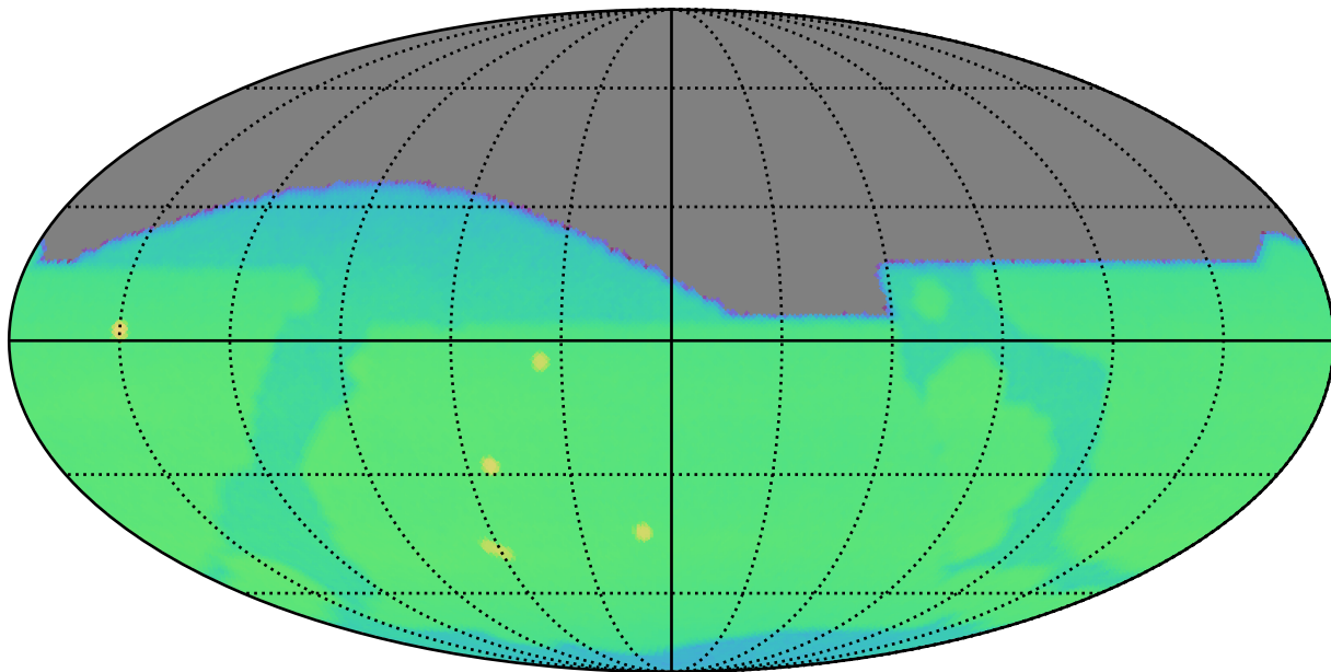
weather_cloudso1v3.4_10yrs : CoaddM5
