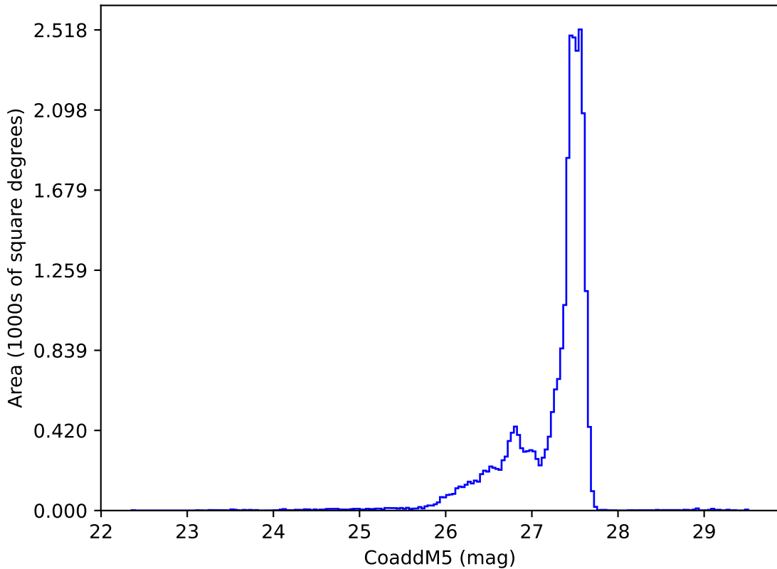
weather_cloudso1v3.4_10yrs : CoaddM5
