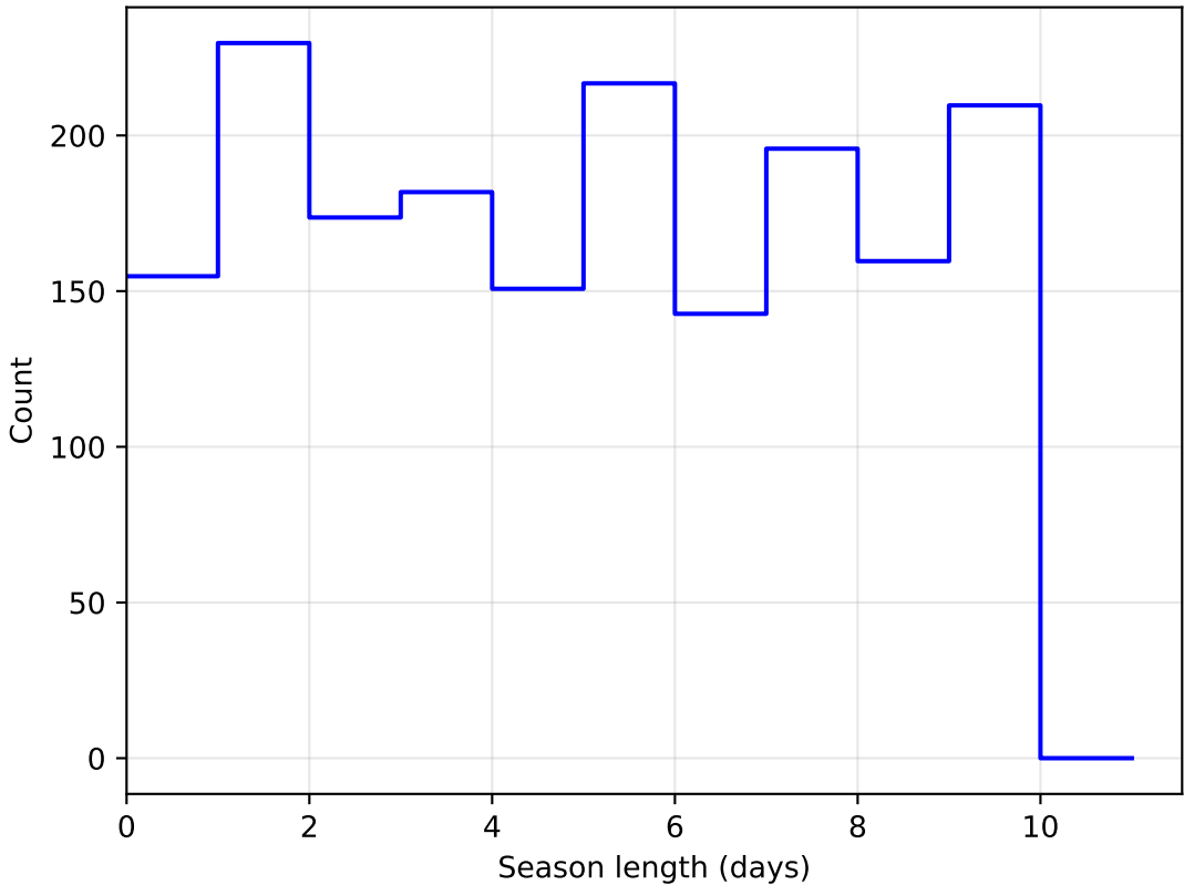
weather_cloudso1v3.4_10yrs DD:WFD all bands: SeasonLength
