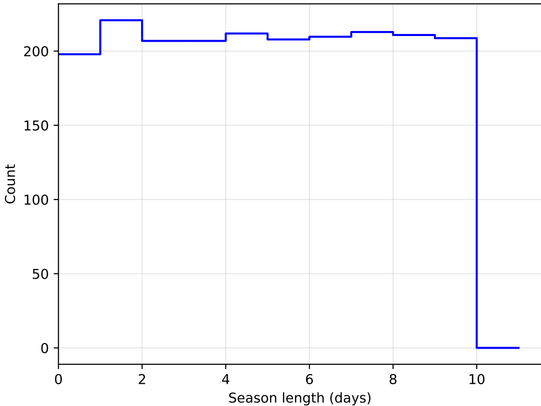
weather_cloudso1v3.4_10yrs DD:ELAISS1 all bands: SeasonLength
