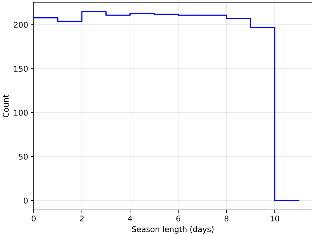
weather_cloudso1v3.4_10yrs DD:EDFS all bands: SeasonLength
