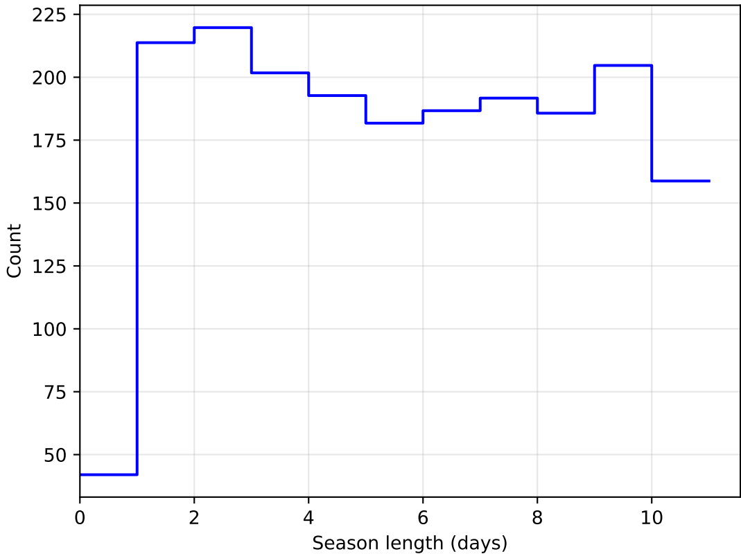
weather_cloudso1v3.4_10yrs DD: COSMOS all bands: SeasonLength
