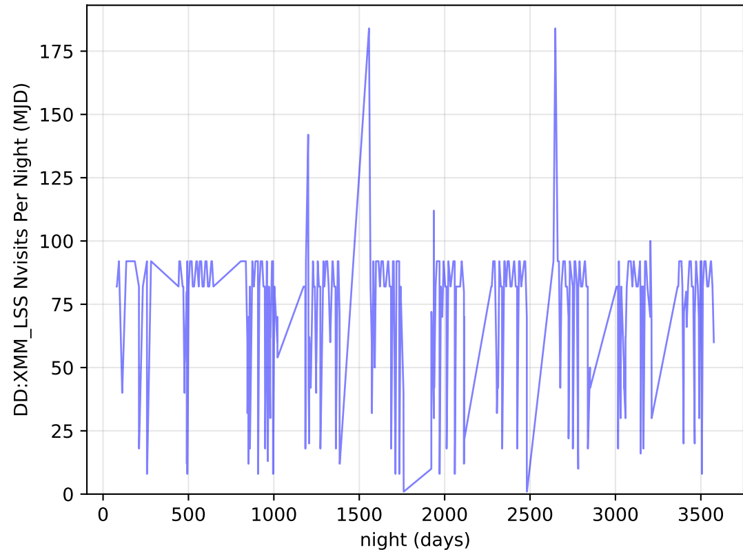
weather_cloudso1v3.4_10yrs all bands: DD:XMM_LSS Nvisits Per Night
