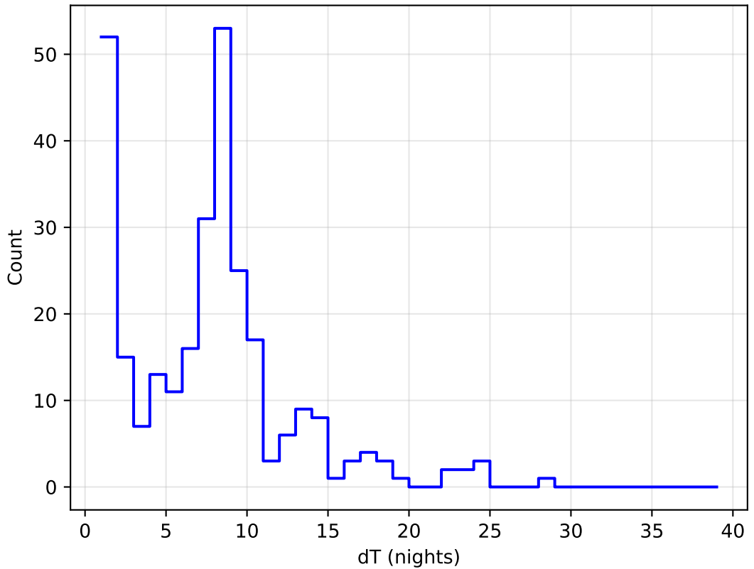
weather_cloudso1v3.4_10yrs all bands: DD:XMM_LSS Delta Nights Histogram
