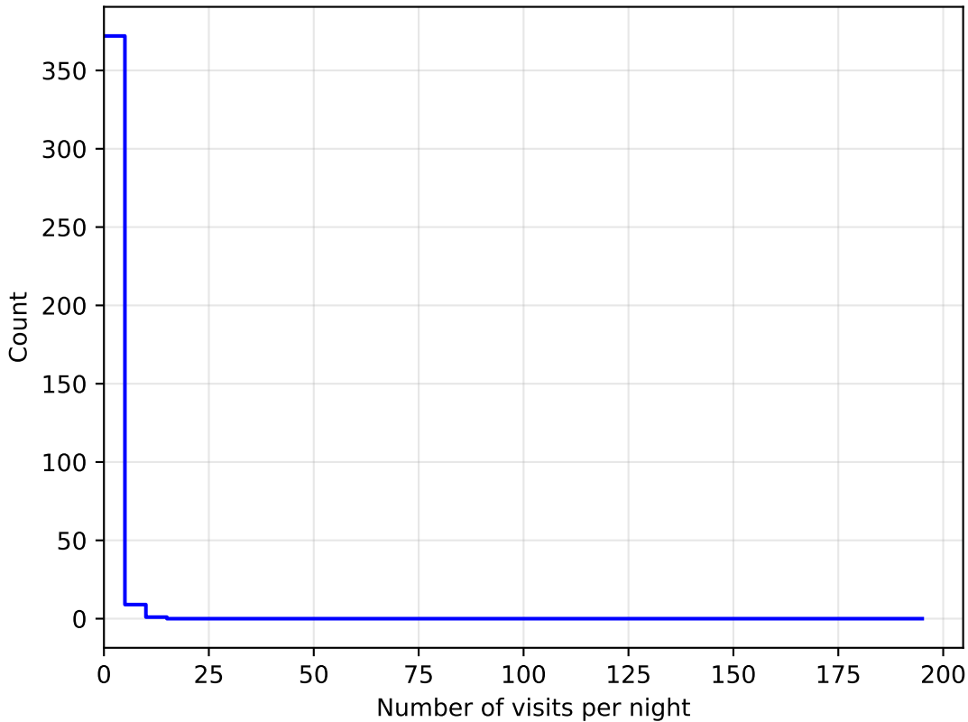
weather_cloudso1v3.4_10yrs all bands: DD:WFD NVisitsPerNight
