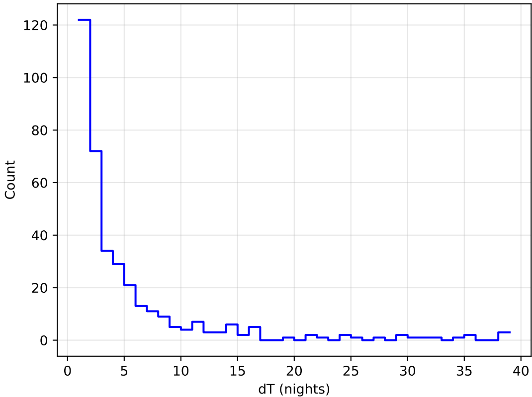
weather_cloudso1v3.4_10yrs all bands: DD:WFD Delta Nights Histogram
