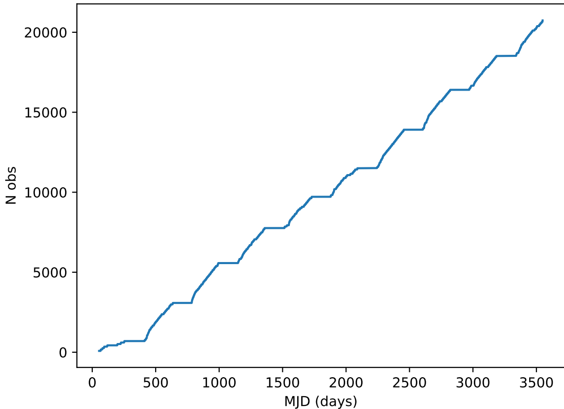
weather_cloudso1v3.4_10yrs all bands: DD:ELAISS1 Cumulative NVisits
